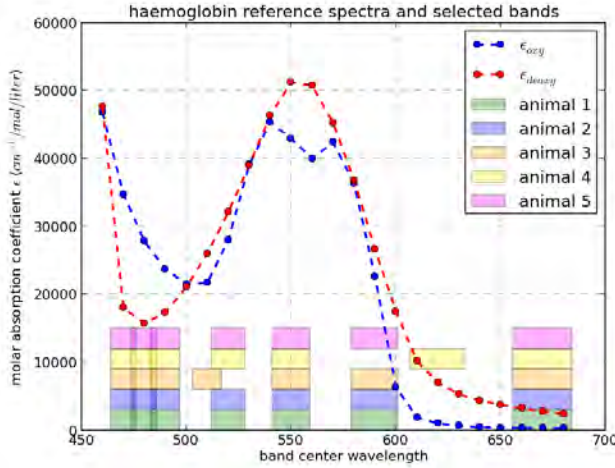
Figure 6.5: The oxy- and deoxy-hemoglobin absorption curves with LCTF responses taken into account. Also indicated are the chosen bands with their respective center wavelength and full widths at half maximum (FWHM). The legend denotes which animal has been left out from training. Reprinted with permission from Wirkert et al. [194].
