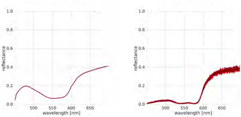
(a) The spectrum with the worst SNR ( 10^6 photons)
