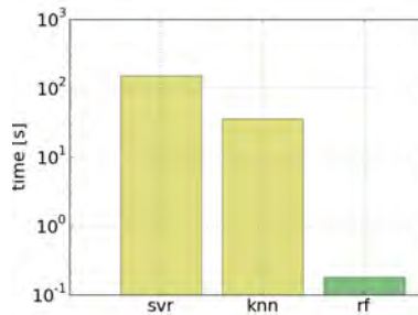
Figure 4.14: Mean computation time for estimation of oxygenation for a multispectral imaging stack of dimension 1,000 \times 1,000 \times 8 , where eight is the number of spectral bands used. Compared are the proposed random forest approach (rf), Support Vector Regression (svr) and k-nearest neighbors (knn). Reprinted with permission from Wirkert et al. [195].
