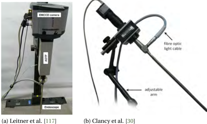
Figure 3.1: Two staring systems that filter light at the camera level. (a) The highly sensitive, but bulky EMCCD camera and the fast switching AOTF allow relatively fast recording of eight bands in 5Hz. (b) The slow switching LCTF and standard monochrome camera record an image stack in about 3s, but feature a smaller form factor. Pictures adapted with permission from [117] and [30].
