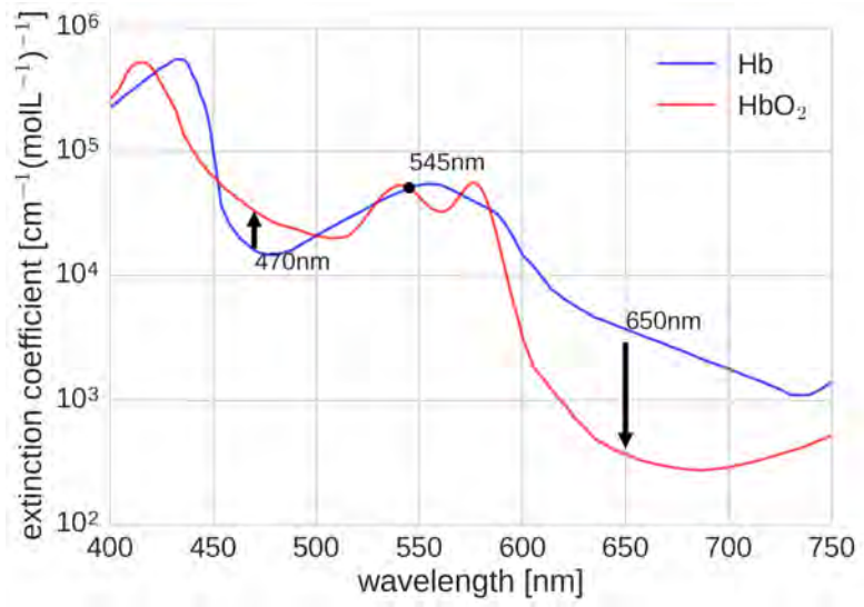
Figure 2.4: Oxygenated ( \text{HbO}_2 ) and deoxygenated ( \text{Hb} ) blood absorb light differently depending on wavelength. This is shown for capillaries of 9\mu\text{m} diameter in (a) and (b). This wavelength dependent absorption is the key to functional imaging. It can further be seen why blood appears red: most light is absorbed in the blue and green wavelength range. The absorption of hemoglobin is determined by the extinction coefficients [152] shown in (c). Light at 545\text{nm} is absorbed the same for both variants, a so called isosbestic point. Although the extinction coefficient technically includes both scattering and absorption, absorption dominates scattering in hemoglobin [191].
