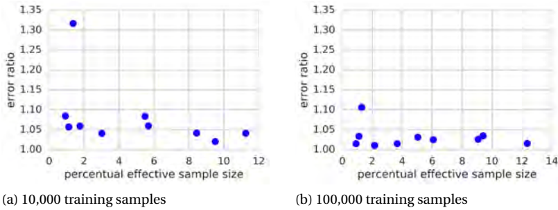
Figure 5.6: Investigation of doubly robust domain adaptation (DR DA) compared to DA without DR correction as a function of effective sample size. The y-axis show the quotient of domain adaptation and doubly robust domain adaptation RMSE.
