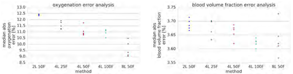
(a) Median oxygenation estimation results for each of the five runs
