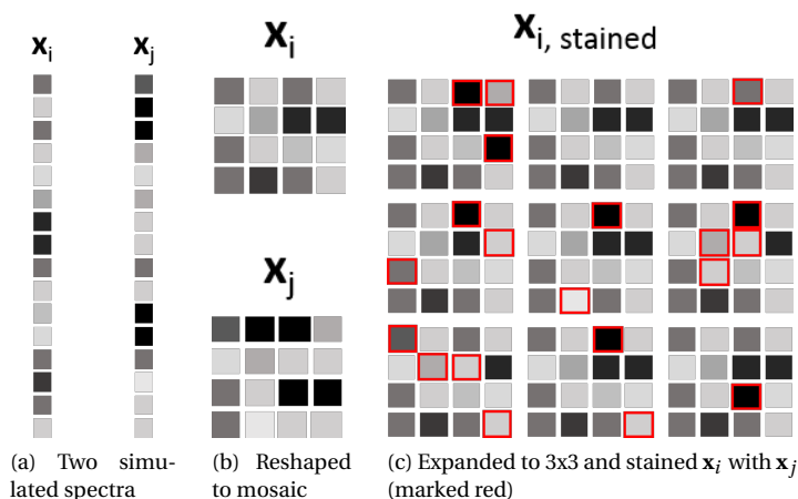
Figure 7.6: Instead of performing regression on single pixels, the presented approach takes into account small neighborhoods. Within this neighborhood the tissue can change. (a) To simulate these spatial changes in tissue, for each simulated sample x_i a random “staining sample” x_j was selected. (b) Both are reshaped into the mosaic pattern recorded by the sensor. (c) Elements of x_i were replaced by elements of x_j with a certain probability. Replaced elements are indicated with a red border in this example. The process of rearrangement and staining was repeated 3 \times 3 = 9 times to form a small simulated patch of data. Figure 7.15 shows the effect of this procedure.
